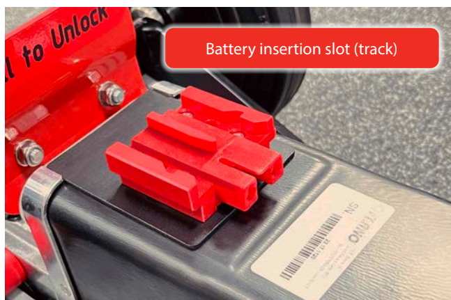
Battery holder on the track motor
